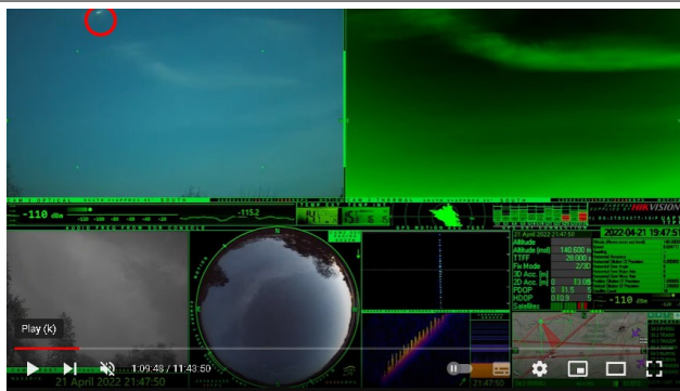
3) Slow moving
